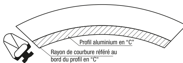
Figure "B" | Pour bords sensibles type "B1NC" - "B1NC-AG" - "B2C" - "B2C-AG" - "B0C" - "B0C-AG"
